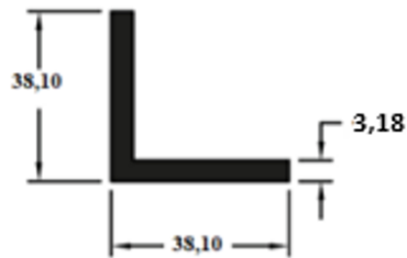
CANT 1.1/2" X 1/8"
