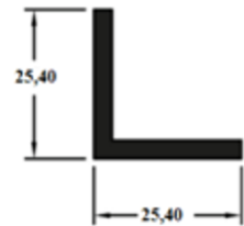
CANT 1"
