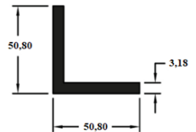
CANT 2" X 1/8"
